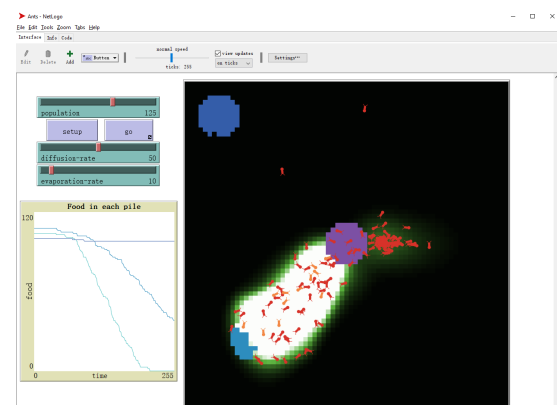
Figure 1: The original Ants model
