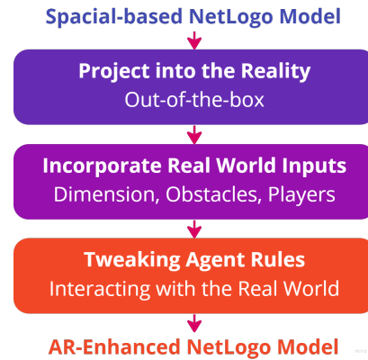
Figure 3: Steps to transform NetLogo models into AR
